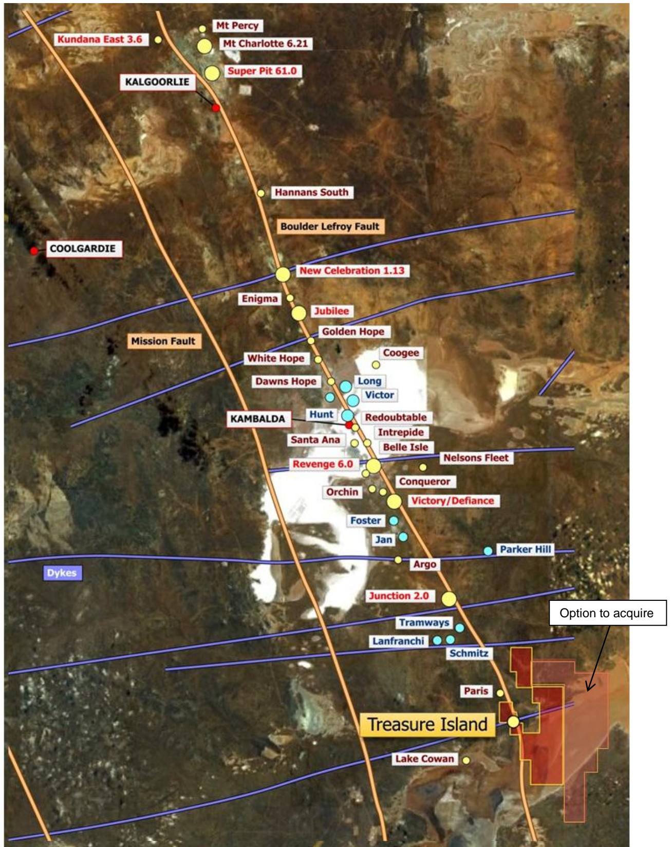
Figure 1: Location of the Treasure Island Gold Project on the Boulder Lefroy Fault
